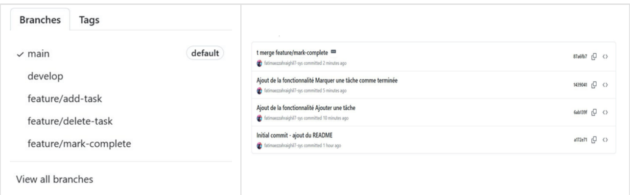
Fig. 3 — Branches GitHub
